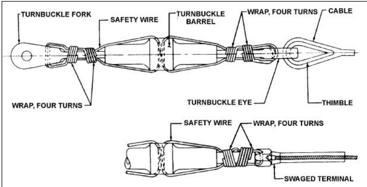
FIGURE 7-25. Securing turnbuckles.
