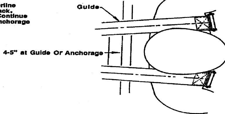
Figure 1-1 Geometry of Shoulder Harness Restraint System
